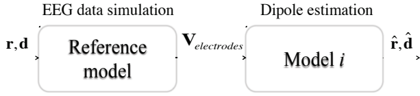
Figure 2. Schematic diagram of the simulation setup.
